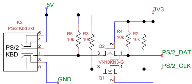
LEVEL SHIFTER
